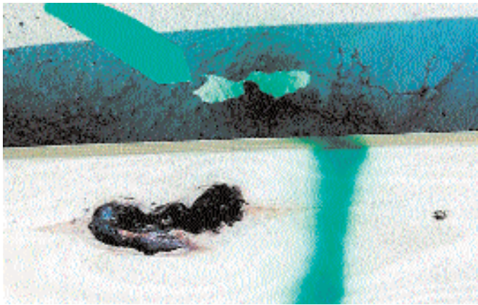
2x6 Chord Using #2 Lumber Notice Sunlight Through Knot Hole
