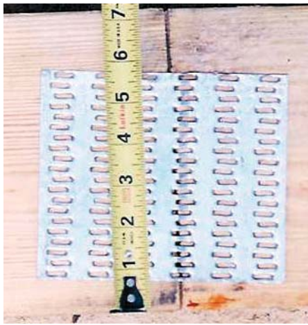
2x8 Chord 5" Metal Connector Plate - Truss is Structurally Adequate - is Very Flexible
