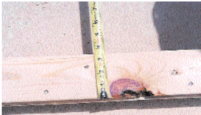
2x4 Chord - #2 Lumber with Knot
